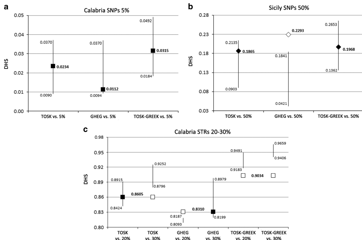
Figure 4 Plots of observed and expected DHS values for fitting scenarios under a stationary model. Evolutionary scenarios with the three putative source populations (Tosks, Gheds and a 50% random blend of Tosks and Greeks) were compared for those models (bold in Table 1) showing at least one fit in the simulations results: (a) Calabria SNPs 5%, (b) Sicily SNPs 50% and (c) Calabria STRs 20–30%. The SD intervals of the simulated distributions are represented by vertical bars. Observed DHS values are represented by symbols filled in black or white depending on whether or not they match the simulated intervals. Squares and diamonds stand for Calabrian and Sicilian Arbereshe, respectively.
